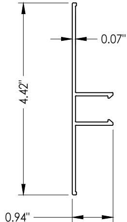
8 JAMB COVER
