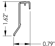
13 SILL CLADDING
