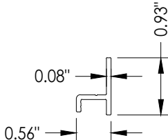
55 WATER BAR
