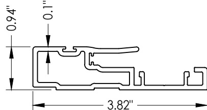
61 WALL HOOK
