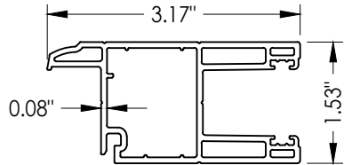
5 STILE & RAIL
