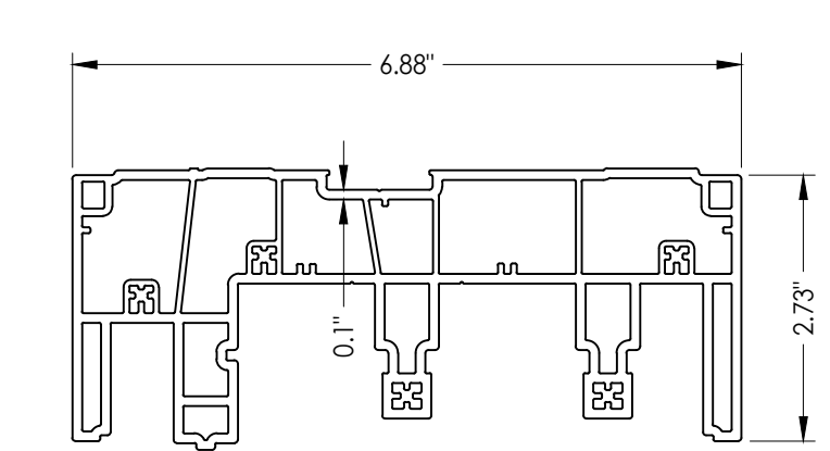
1 FRAME HEAD
