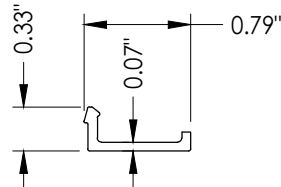
28 GLAZING BEAD
