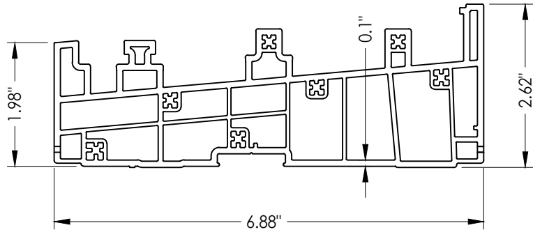
12 FRAME SILL
